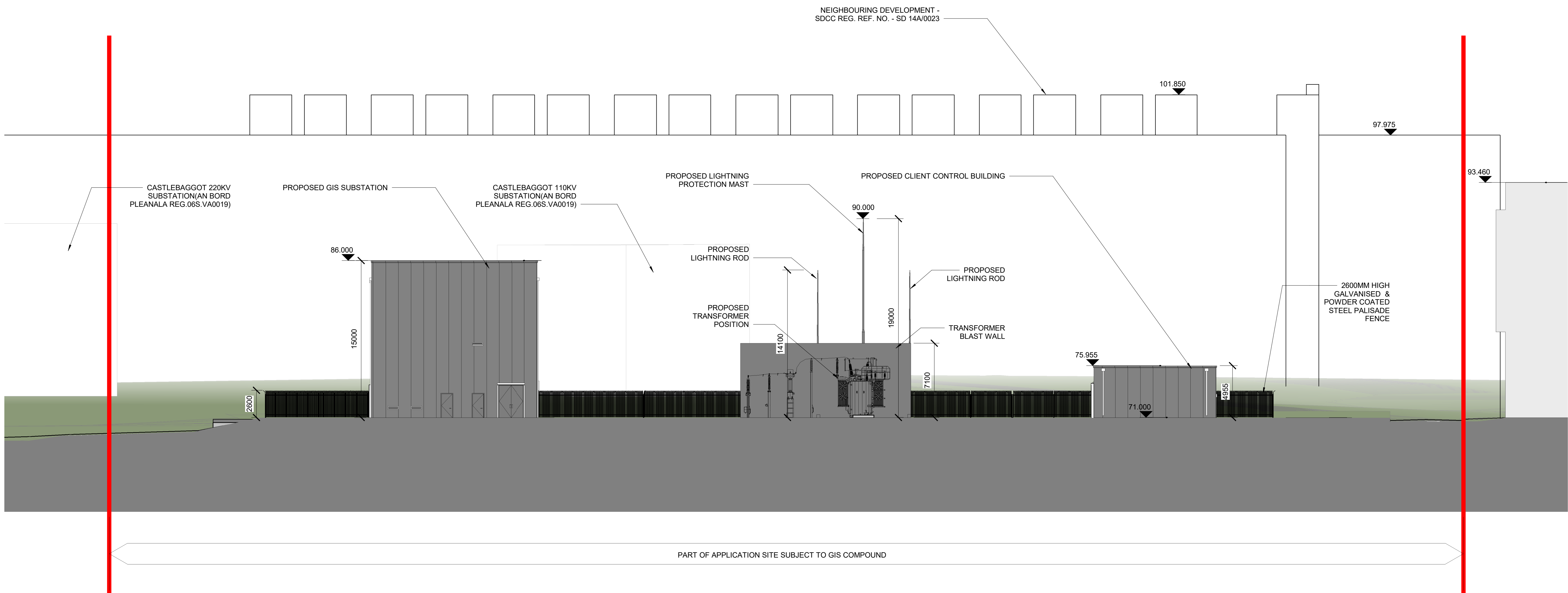
2 PROPOSED COMPOUND SECTION 2-2 1 : 200
