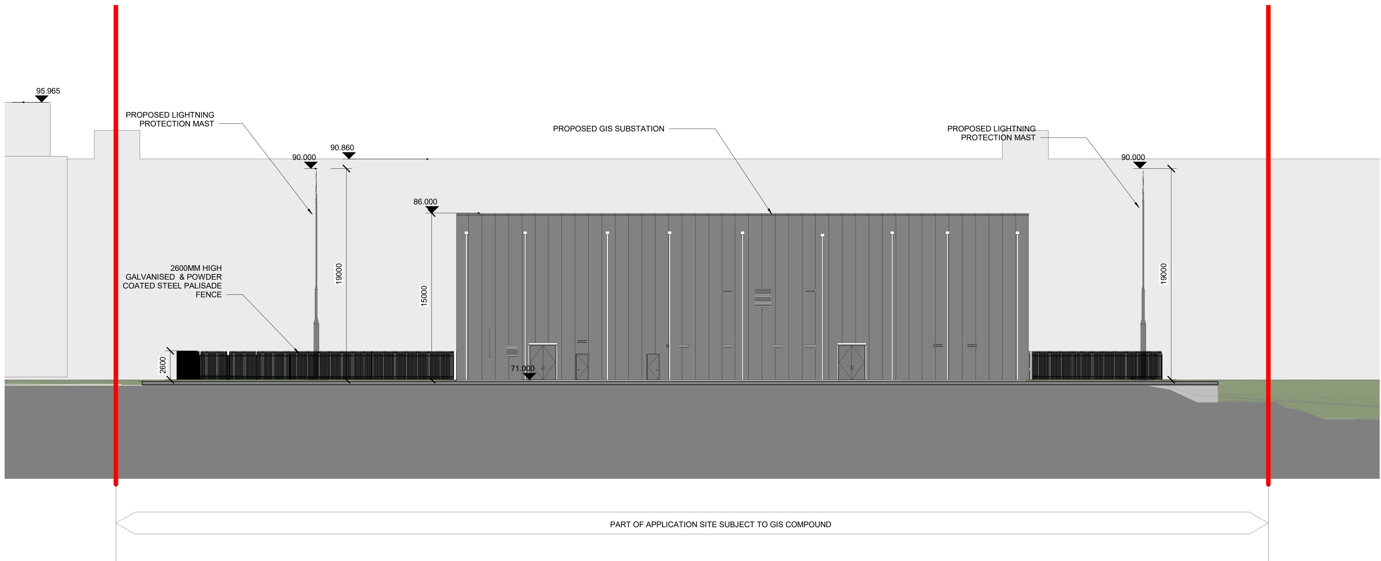
1 PROPOSED COMPOUND SECTION 1-1 1 : 200
